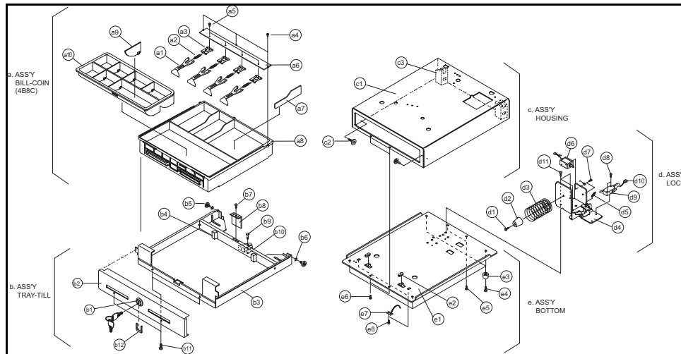
Figure9-13 Drawer (4B/8C)
