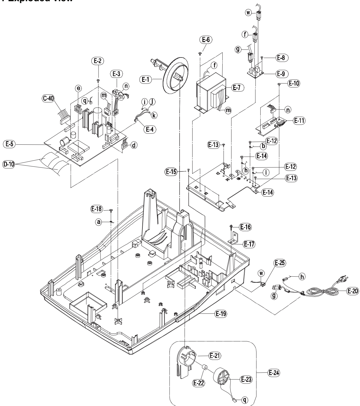
Figure9-7 Case Lower Assembly
