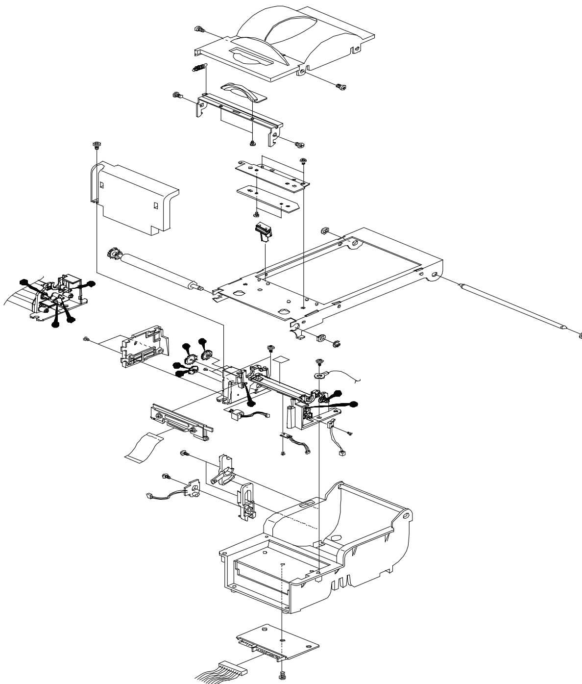
Figure9-5 Lubrication Points of the Printer (STM-210)
