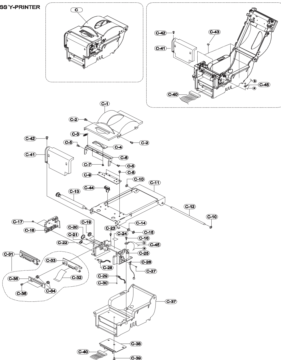
Figure9-4 Printer (STM-210)
