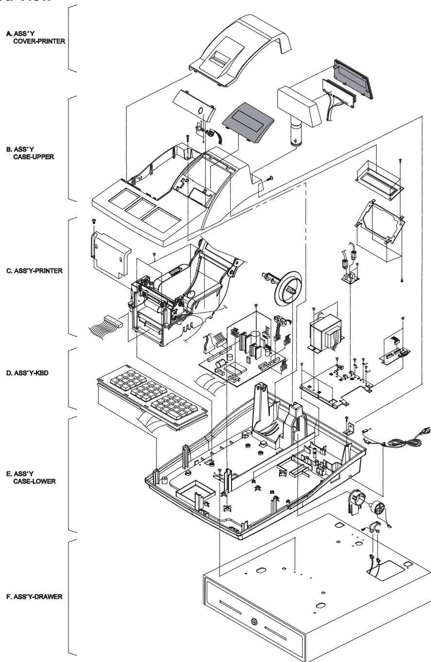
Figure9-1 Total Disassembly
