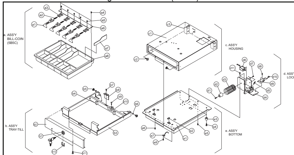
Figure9-14 Drawer (5B/5C)
