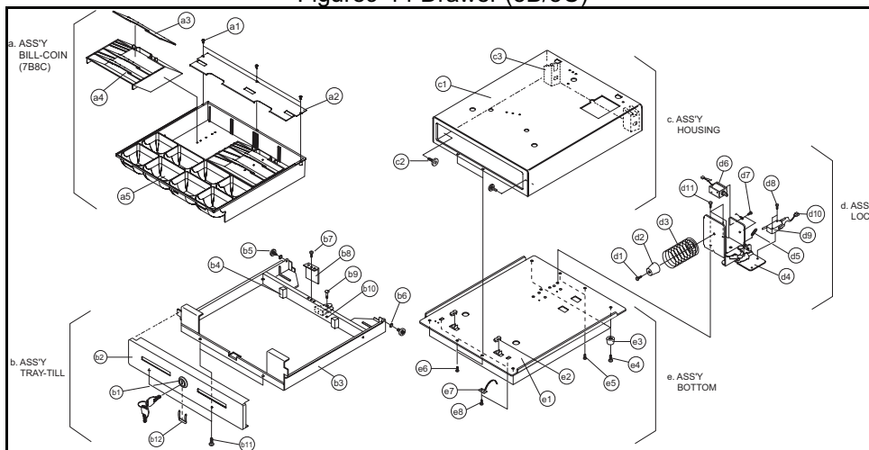
Figure9-15 Drawer (7B/8C)
