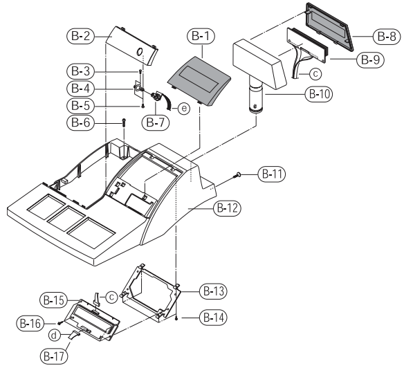
Figure9-3 Case Upper Assembly
