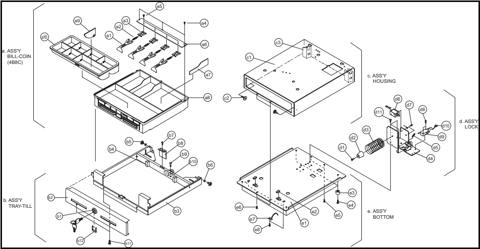
Figure7-9 Drawer (4B/8C)
