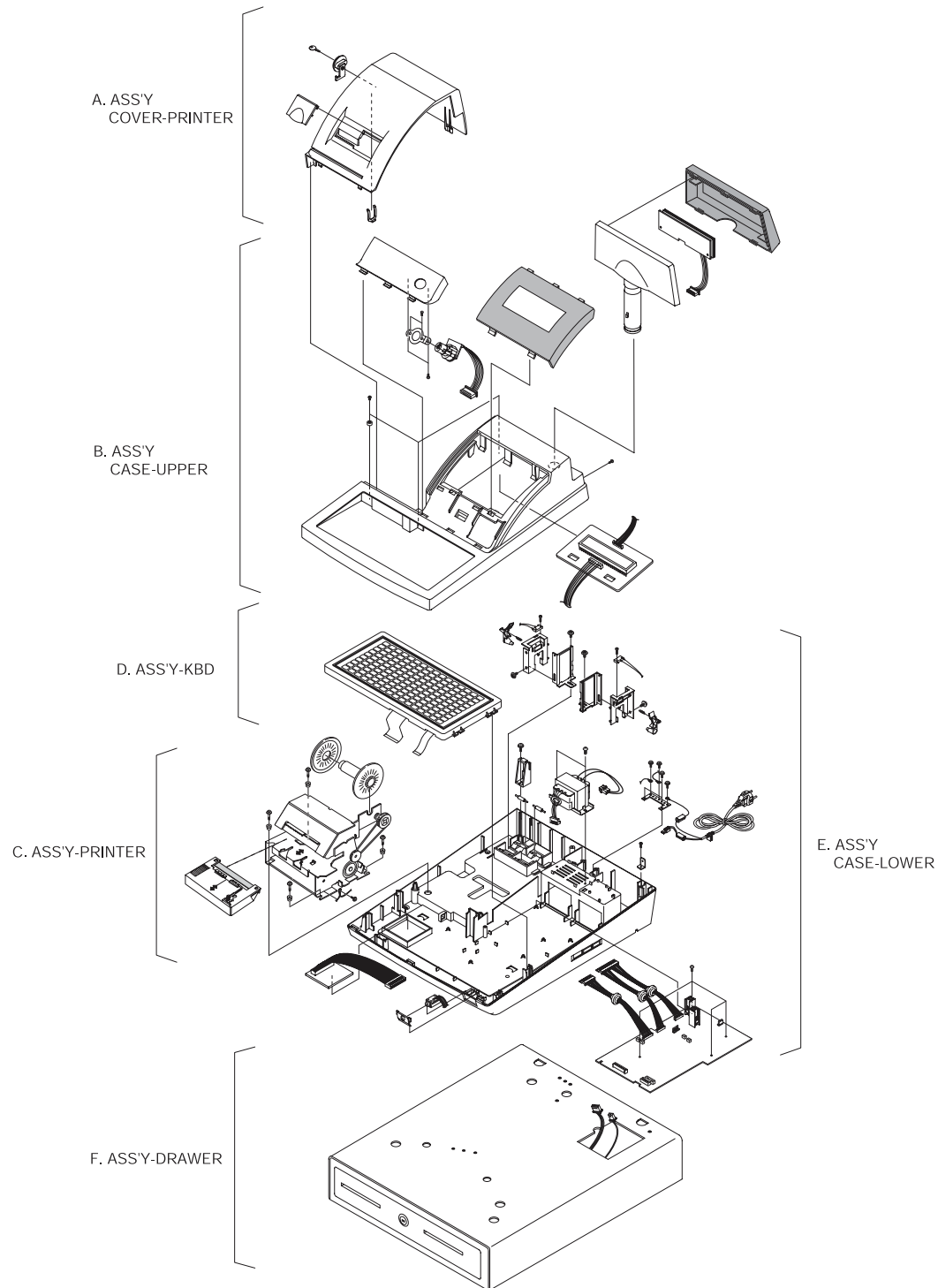
Figure7-1 Total Disassembly
