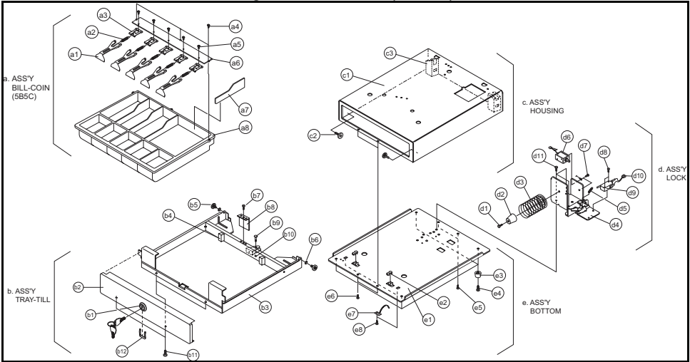
Figure7-10 Drawer (5B/5C)
