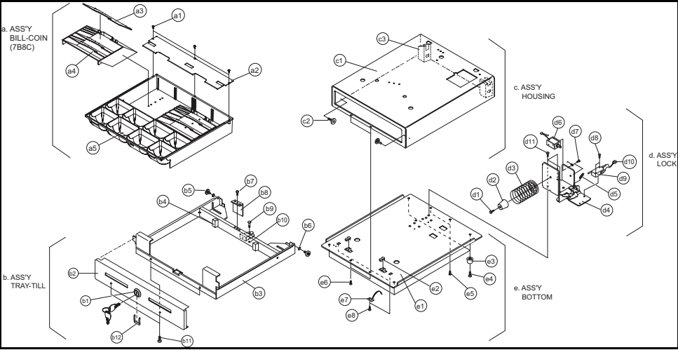
Figure7-11 Drawer (7B/8C)
