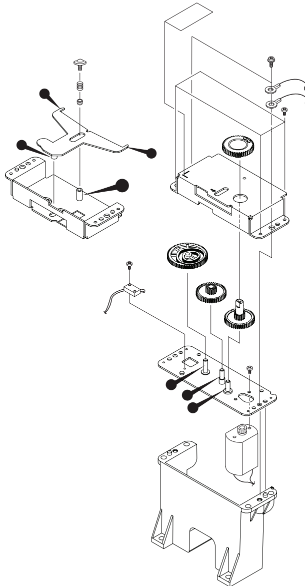
Figure9-10 Lubrication Points of the Auto-Cutter (SAC-60)
