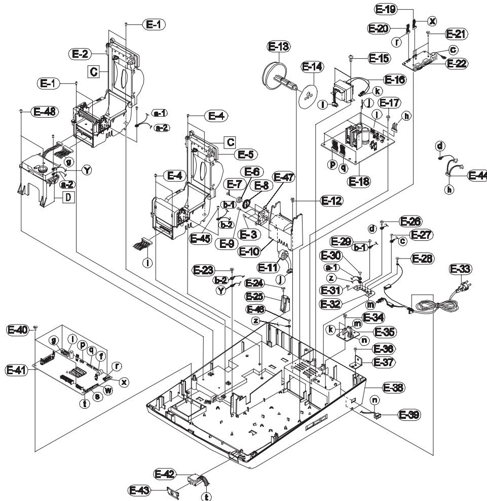
Figure9-6 Case Lower Assembly
