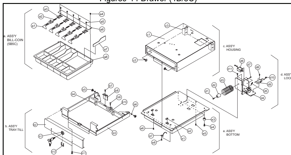
Figure9-15 Drawer (5B/5C)
