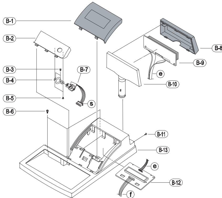
Figure9-5 Case Upper Assembly(ER-5200)
