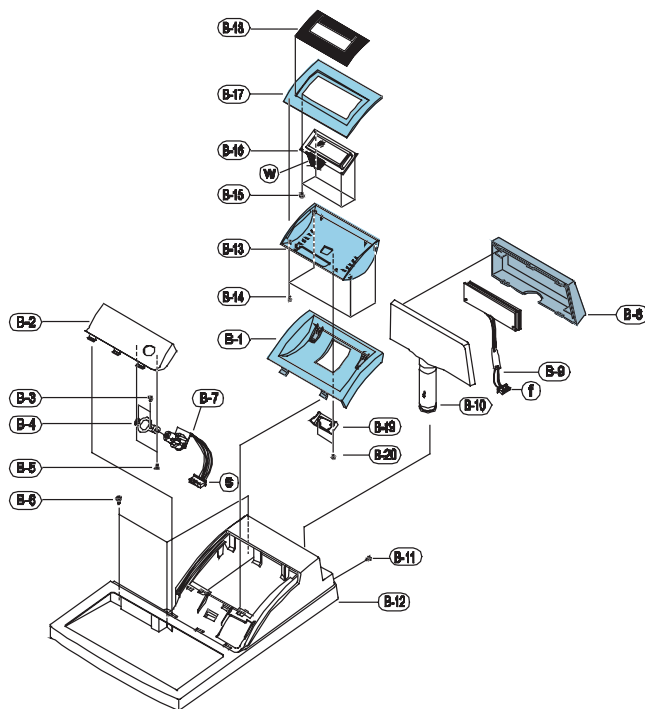
Figure9-4 Case Upper Assembly(ER-5200M)
