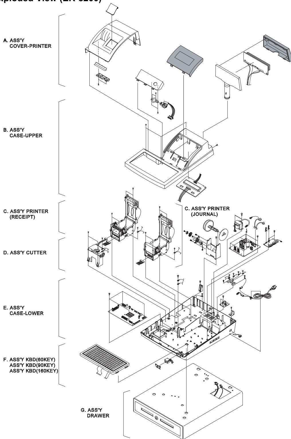
Figure9-2 Total Disassembly
