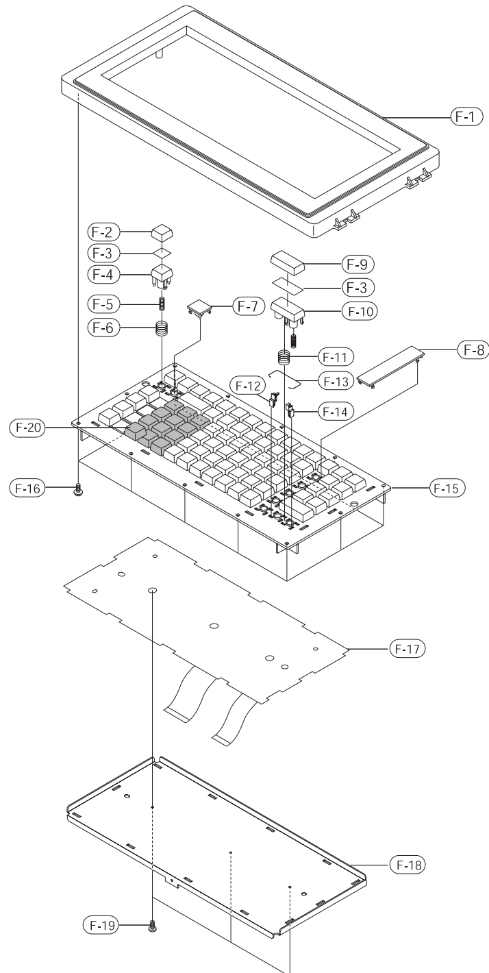
Figure9-12 Key Board (90 Key)
