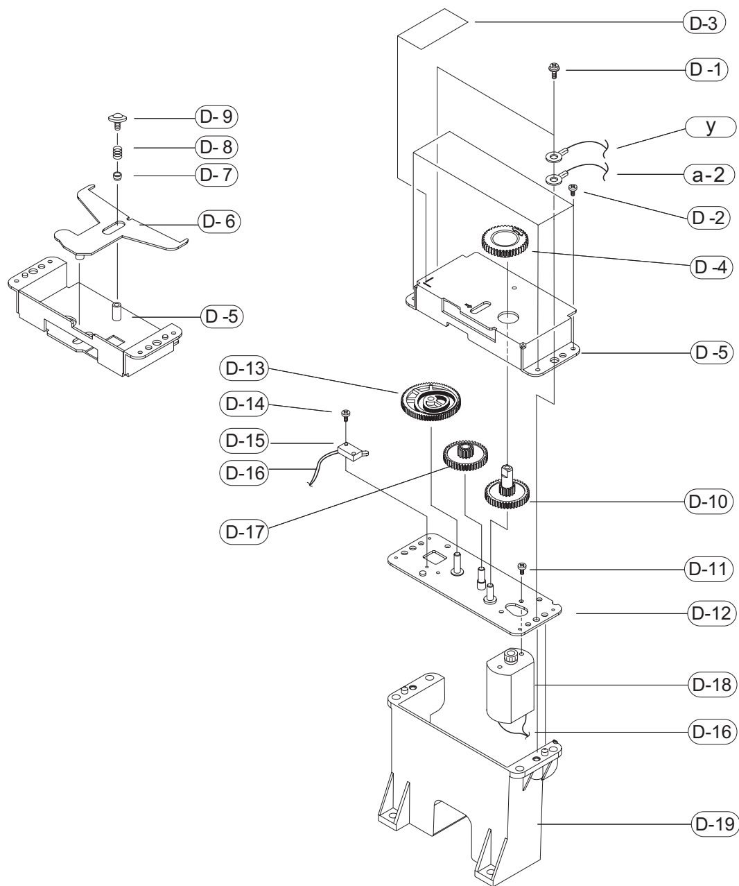
Figure9-9 Auto Cutter (SAC-60)
