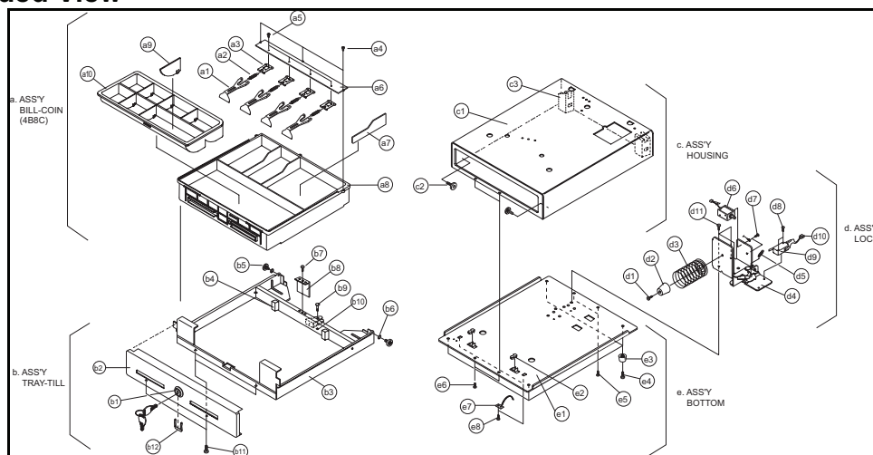
Figure9-14 Drawer (4B/8C)
