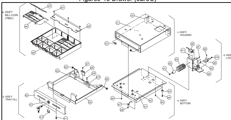
Figure9-16 Drawer (7B/8C)
