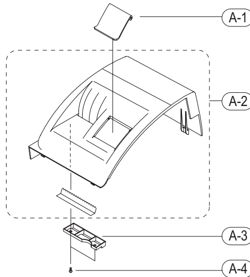
Figure9-3 Cover Printer
