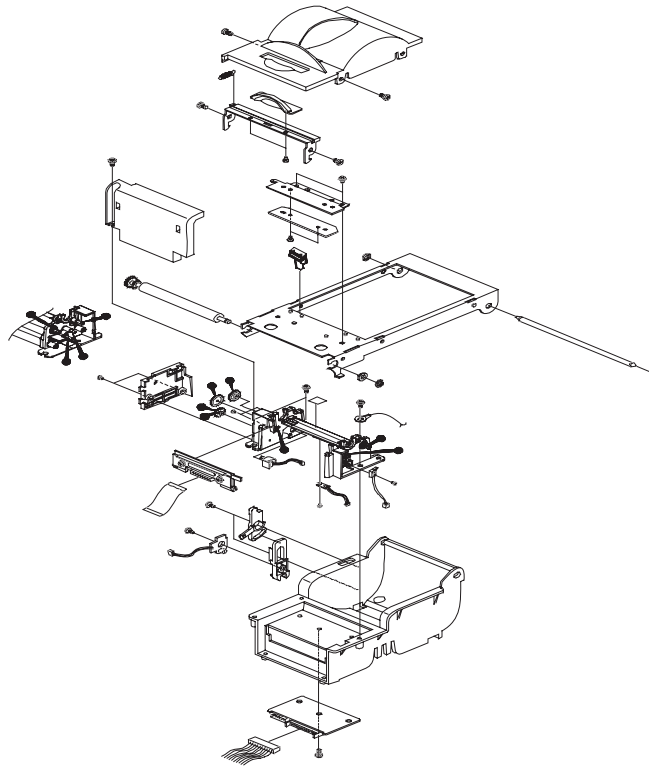
Figure9-8 Lubrication Points of the Printer (STM-210)
