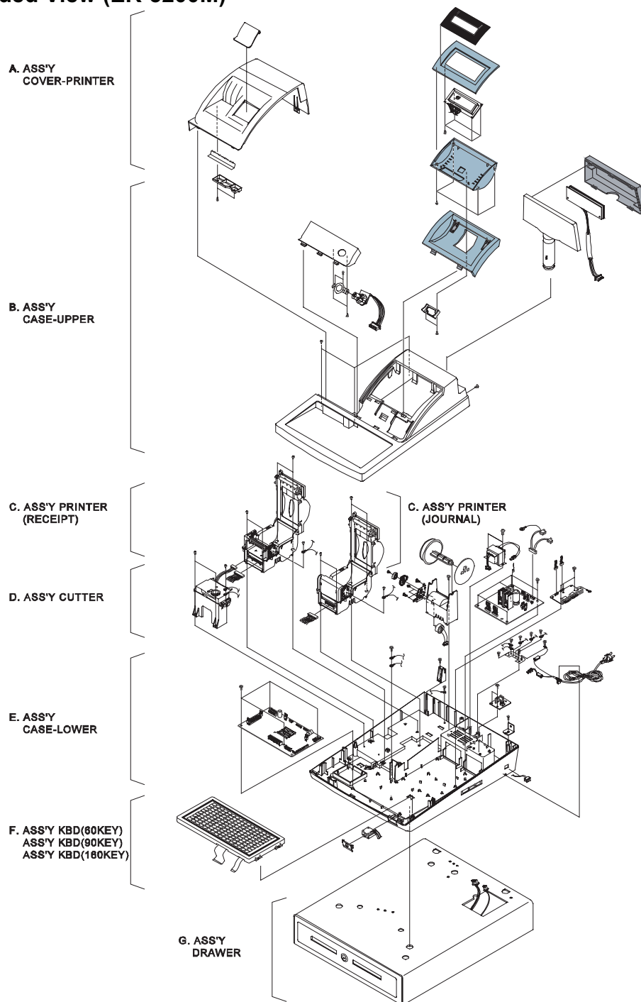
Figure9-1 Total Disassembly
