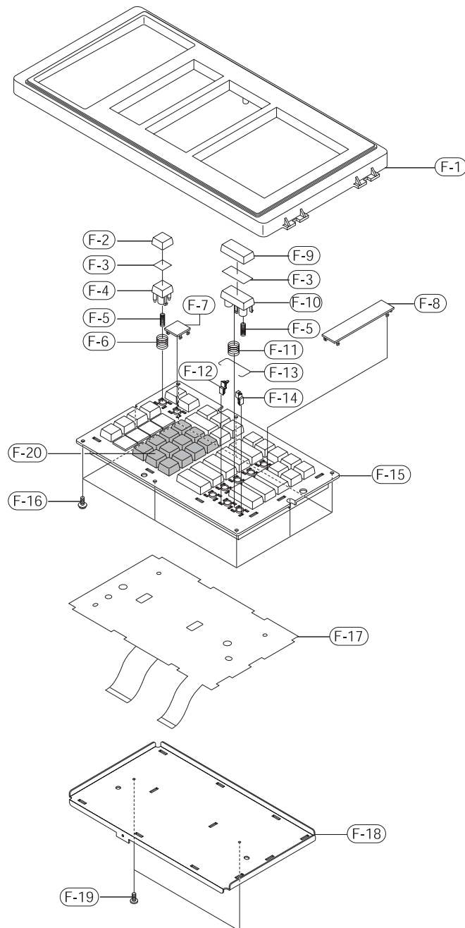
Figure9-11 Key Board (60 Key)
