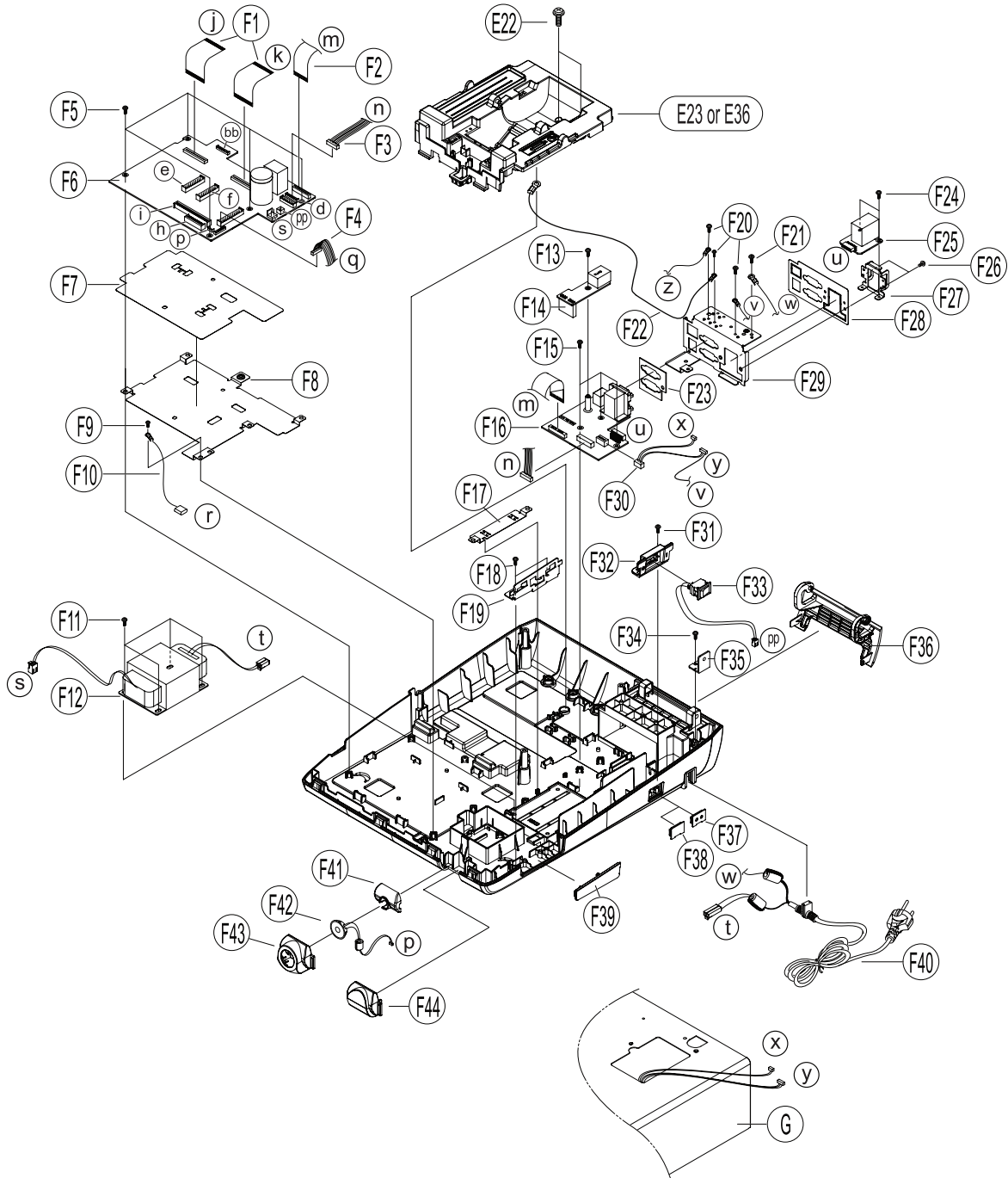
Figure7-14 ASS'Y-CASE LOWER
